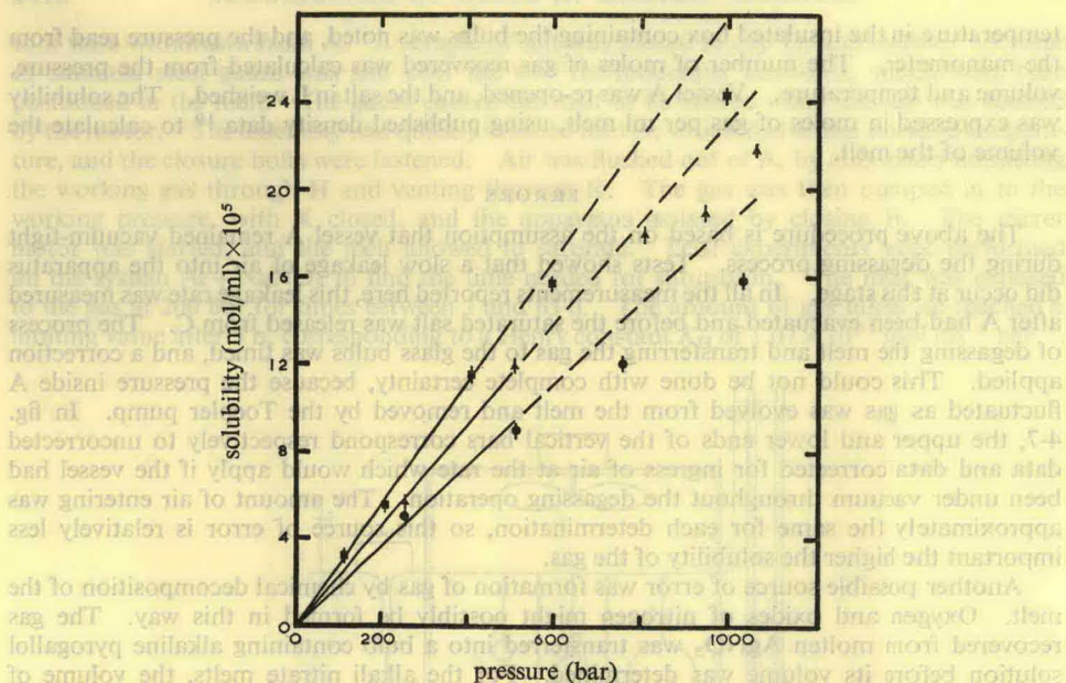
FIG. 4(a).—Solubility isotherms for the system He+NaNO 3 . ■, 441°C; ▲, 391°C; ●, 332°C.
